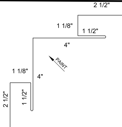
Inside Corner Post
